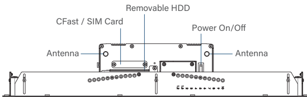
Front I/O
